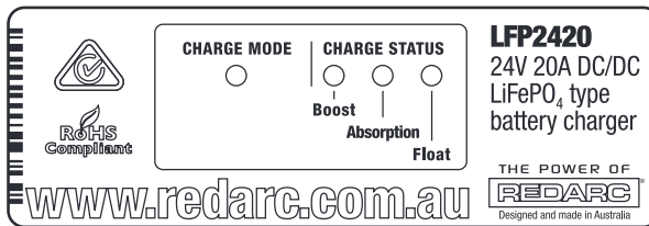
Figure 1.1 - The LFP2420(-LV) Front Panel
